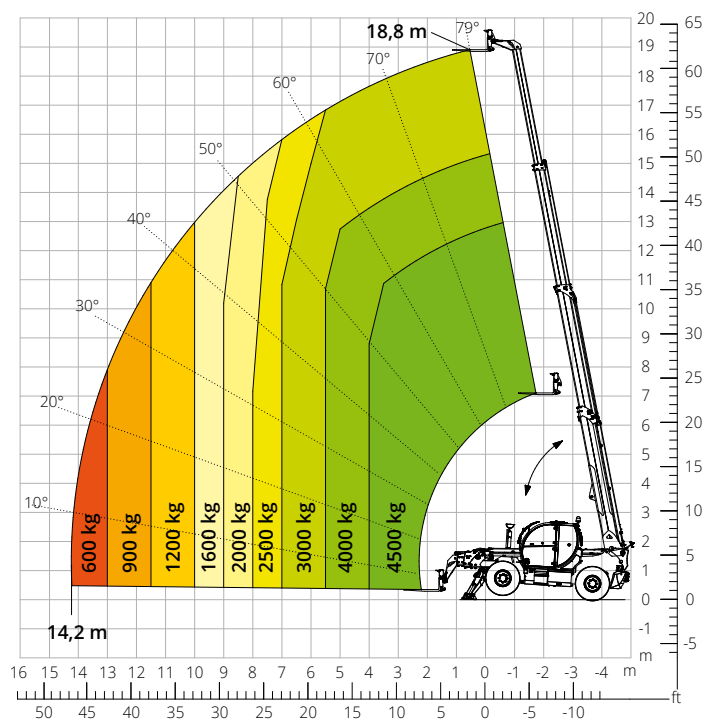
Load chart with FULLY EXTENDED STABILISERS ATT-03-042
