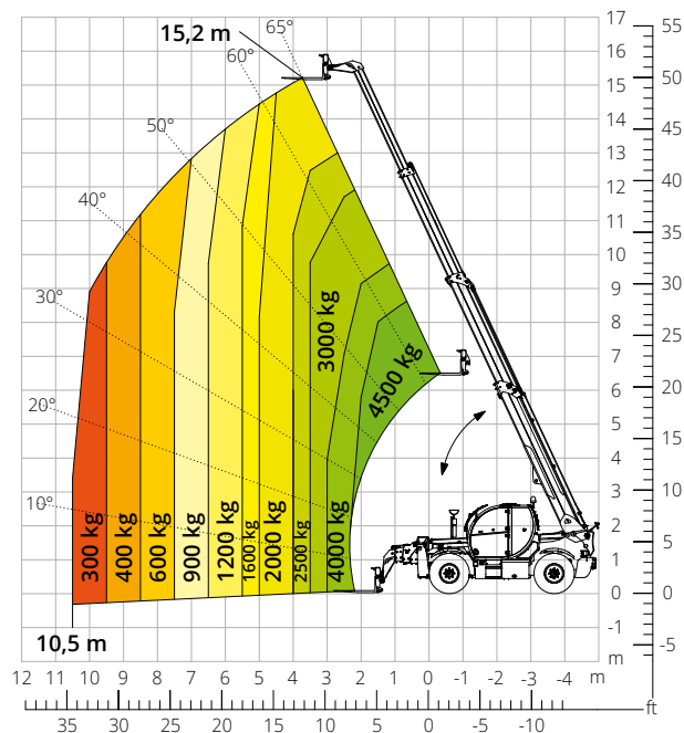
Load chart with WINCH, 5,000 kg ATT-02-019
