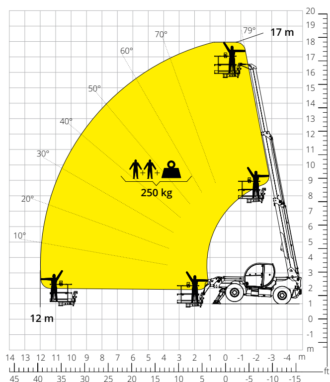
Load chart with ROTATING NON-EXTENDABLE PLATFORM, 250 kg ATT - 01 - 003
