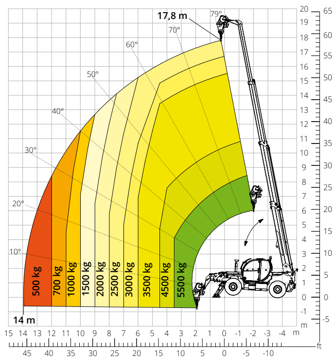
Load chart with WINCH, 6,000 kg ATT-02-004
