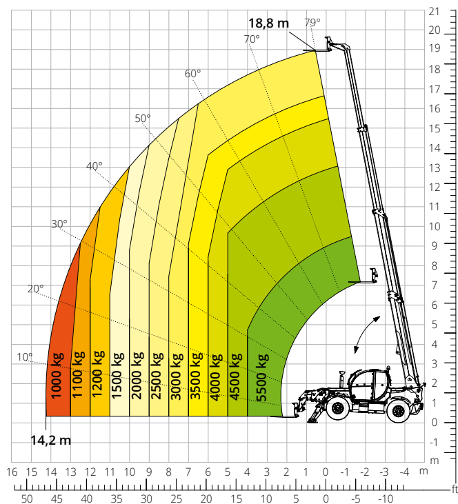
Load chart with FULLY EXTENDED STABILISERS ATT-03-040
