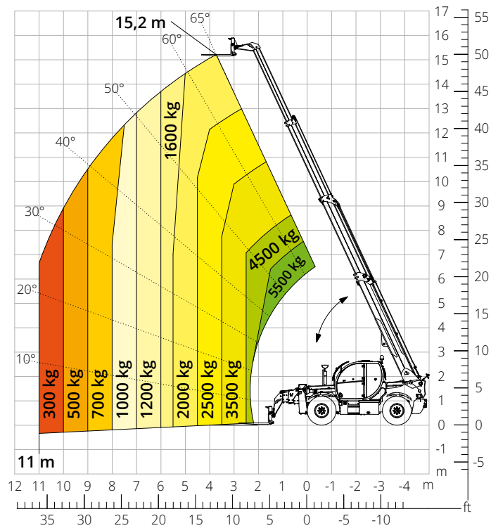
Load chart FRONT ATTACHMENT ON TYRES ATT-03-040
